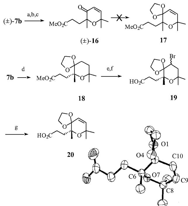
Scheme 3. Elaboration of the pyran core and ORTEP drawing of the crystal structure of 20 : a) TMSCl, Et 3 N, DMF, 12 h, 100 °C, 87%; b) Br 2 , CCl 4 , 0 °C, 77%; c) LiBr, Li 2 CO 3 , DMF, 100 °C, 12 h, 81%; d) (CH 2 OH) 2 , TsOH, toluene, reflux, 8 h, 84%; e) Br 2 , CCl 4 , 40 °C, 45 min; f) 2 N NaOH, MeOH, 20 °C, 18 h; g) t BuOK, DMSO, 110 °C, 4 h, 75% from 18
