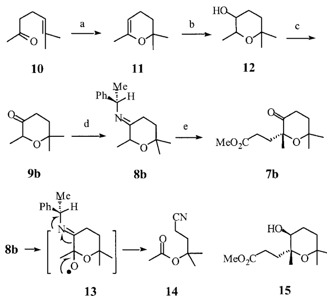
Scheme 2. Enantioselective synthesis of the chiral pyran 7b : a) i : 40% H 2 SO 4 , 20 °C, 45 min, ii : distillation, 85%; b) i : BH 3 ·SMe 2 , cyclohexane, 0 °C, 3 h ii : NaOH, H 2 O 2 , EtOH, 80 °C, 2 h, 93%; (c) i : DMSO, ClCOCl, CH 2 Cl 2 , -78 °C ii : Et 3 N, 68%; d) ( S )-PhCH(Me)NH 2 , 5-Å molecular sieves-SiO 2 -Al 2 O 3 , cyclohexane, 48 h, 20 °C; e) H 2 C=CHCO 2 Me, 48 h, 50 °C, 62% overall from 9b
