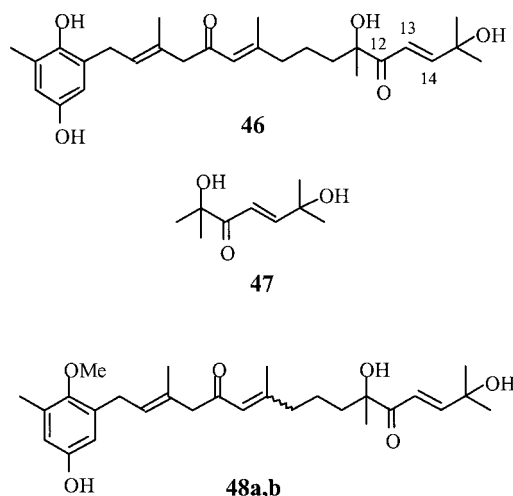
Figure 2. Structure of meroterpenes 51 and putative structures of usneoidones
