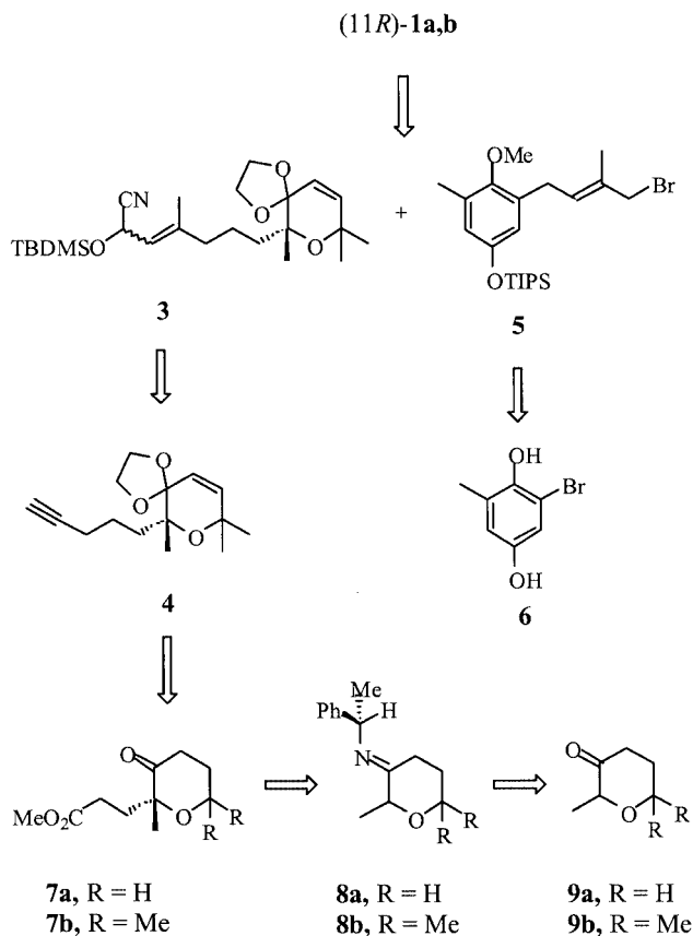
Scheme 1. Retrosynthetic analysis of usneoidones
