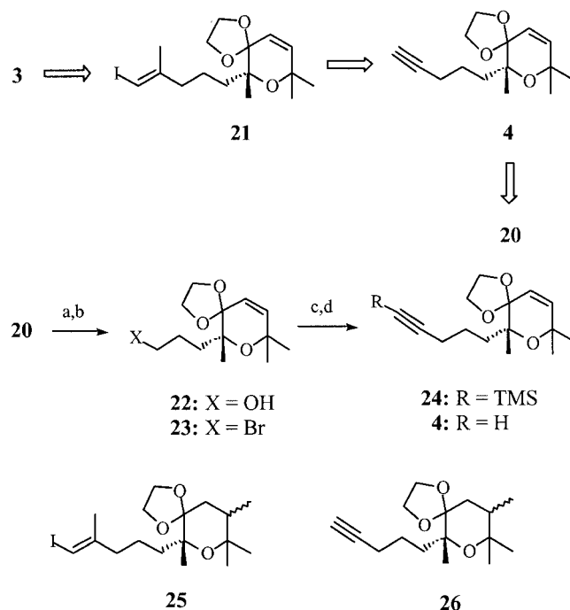
Scheme 4. Attempted functionalization of the side chain through zirconocene-catalyzed carboalumination: a) LAH, Et 2 O, 20 °C, 30 min, 84%; b) CBr 4 , PPh 3 , pyridine, Et 2 O, 4 h, 20 °C, 80%; c) TMSCLi, THF, DMPU, 12 h, 20 °C, 76%; d) n Bu 4 NF, THF, 20 °C, 1 h, 92%
