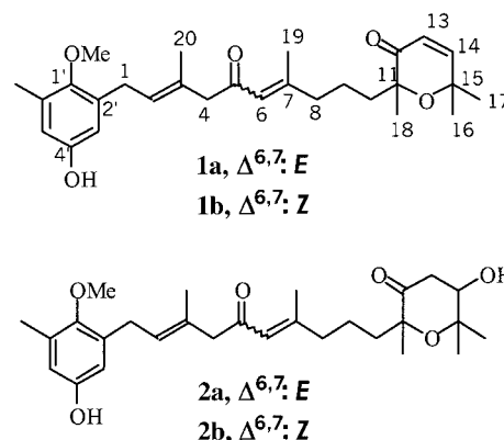
Figure 1. Structures of usneoidones and usneoidols, as proposed by Urones et al.
