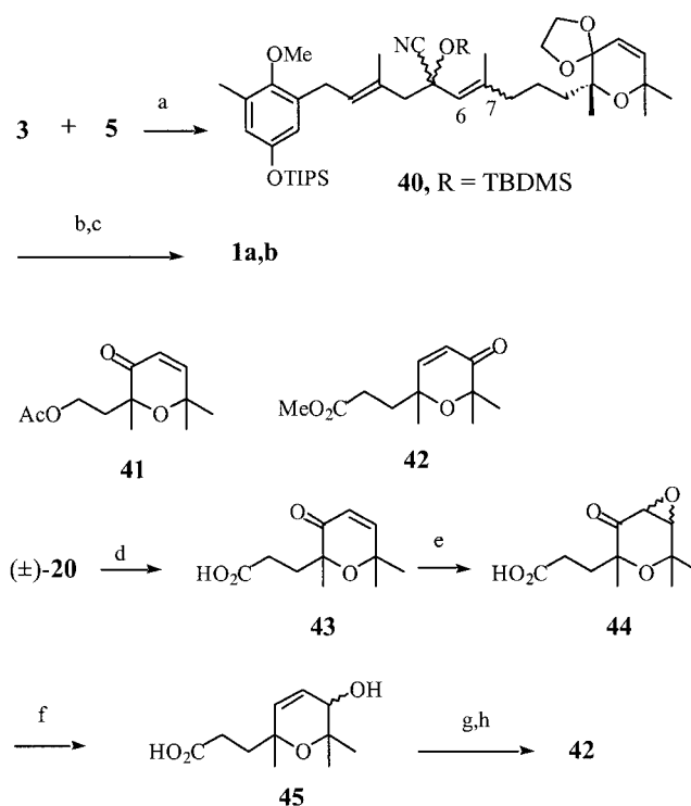
Scheme 7. Completion of the synthesis of 1a,b and Wharton rearrangement of 44 : a) i : LDA, -78^\circ\text{C} , THF, 15 min; ii : 2 equiv. 5 , DMPU, 4 h, 20^\circ\text{C} , 80%; b) 1 M n\text{Bu}_4\text{NF} , THF, 2 h, 20^\circ\text{C} ; c) 0.5 N HCl, THF, 2 h, 20^\circ\text{C} , 64% overall from 40 ; d) 1 N HCl, THF, 1 h, 20^\circ\text{C} , 85%; e) \text{H}_2\text{O}_2 , 1 N NaOH, MeOH, 30 min, 0^\circ\text{C} , 77%; f) \text{H}_2\text{NNH}_2 , MeOH, AcOH, 60^\circ\text{C} , 2 h, 40%; g) Dess–Martin periodinane, \text{CH}_2\text{Cl}_2 , 1 h; h) \text{CH}_2\text{N}_2 , \text{Et}_2\text{O} , 0^\circ\text{C} , 52% from 45
