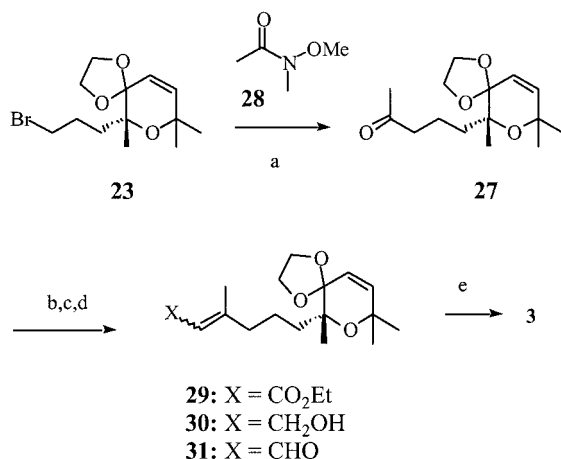
Scheme 5. Elaboration of the side chain of cyanohydrin 3 : a) i : t BuLi, Et 2 O, −78 °C, 15 min, ii : 28 , THF, 3 h, 20 °C, 46%; b) EtO 2 CCH 2 PO(OEt) 2 , n BuLi, THF, 20 °C, 24 h, 83%, ( E )/( Z ) = 4:1; c) DIBAL-H, THF, −70 °C, 2 h, 95%; d) MnO 2 , CH 2 Cl 2 , 20 °C, 8 h, 90%; e) t BuMe 2 SiCN, CH 3 CN, 80 °C, 10 h, 80%
